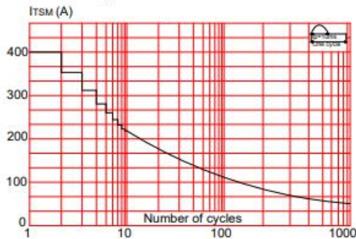
FIG.5: Non-repetitive surge peak on-state current for a sinusoidal pulse with width tp < 10ms, and corresponding value of I't (di/dt < 150A/μs)
