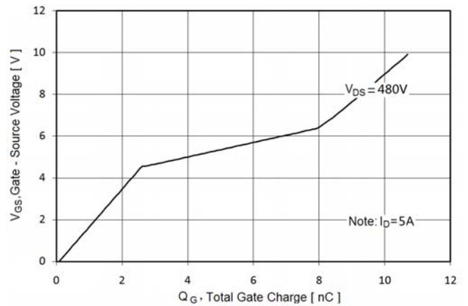
Figure9. Gate charge waveforms
