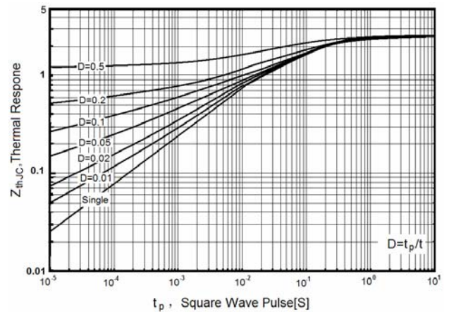
Figure11. Transient Thermal Impedance TO220F
