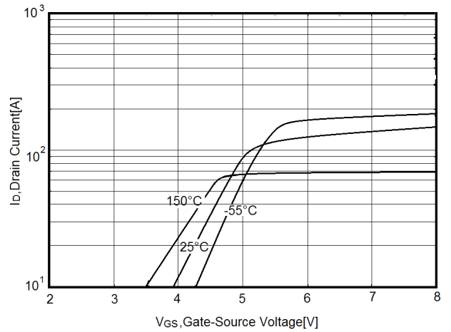
Figure4. Transfer characteristics
