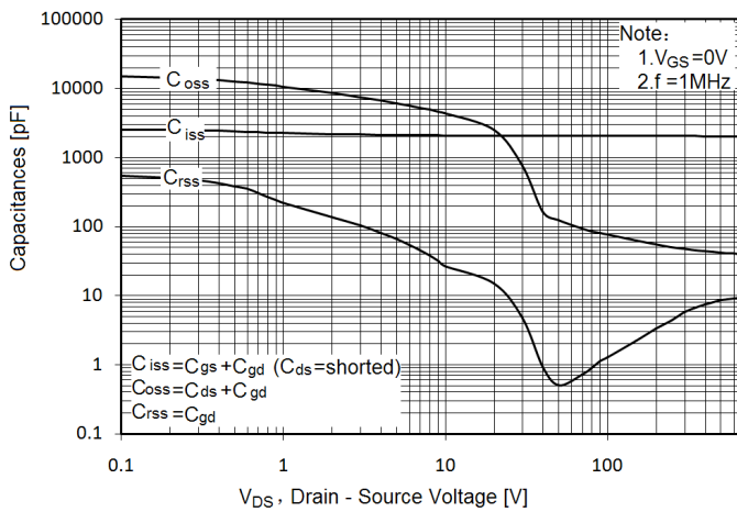
Figure10. Capacitance
