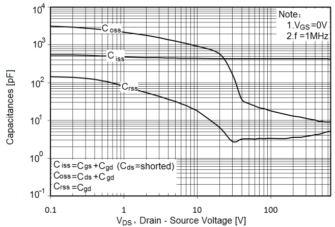
Figure9. Capacitance
