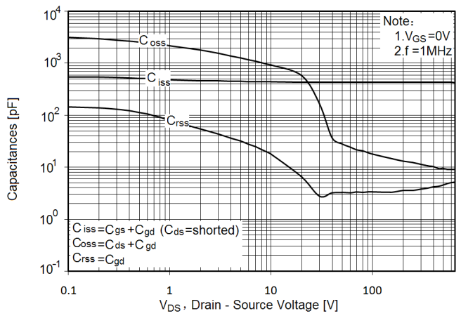
Figure9. Capacitance
