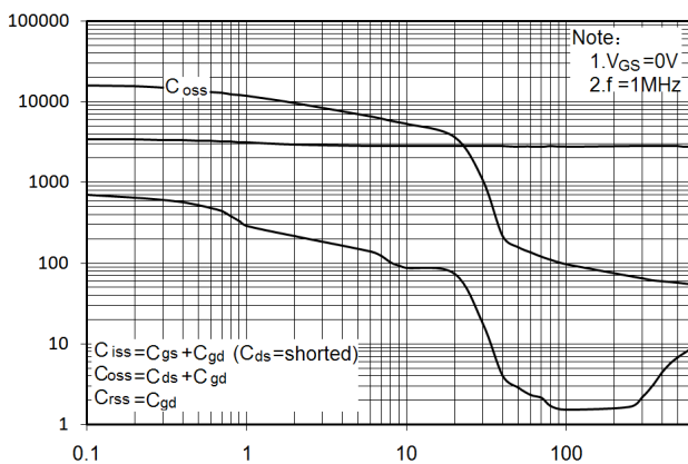
Figure10. Capacitance
