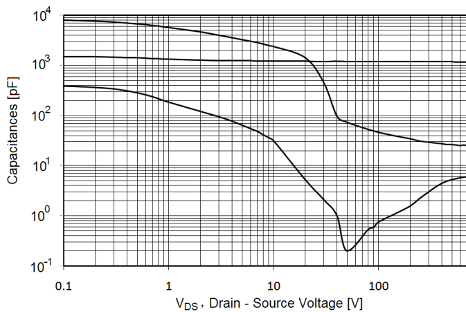
Figure10. Capacitance
