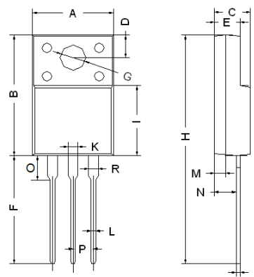
TO-220F
