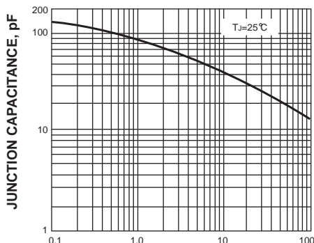
FIG. 5-TYPICAL JUNCTION CAPACITANCE
