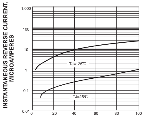
FIG. 4-TYPICAL REVERSE CHARACTERISTICS
