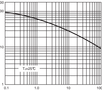
FIG. 5-TYPICAL JUNCTION CAPACITANCE
