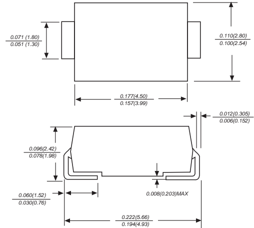
DO-214AC
