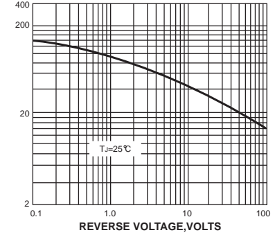
FIG. 5-TYPICAL JUNCTION CAPACITANCE
