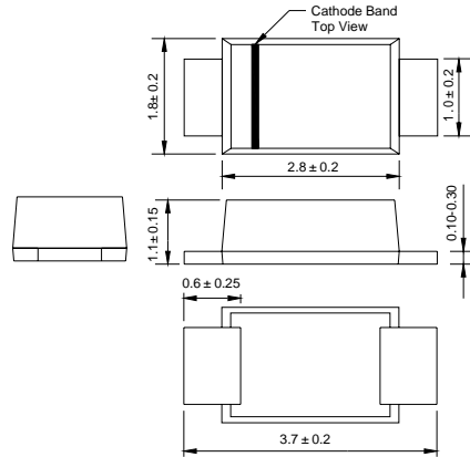
SOD-123FL
